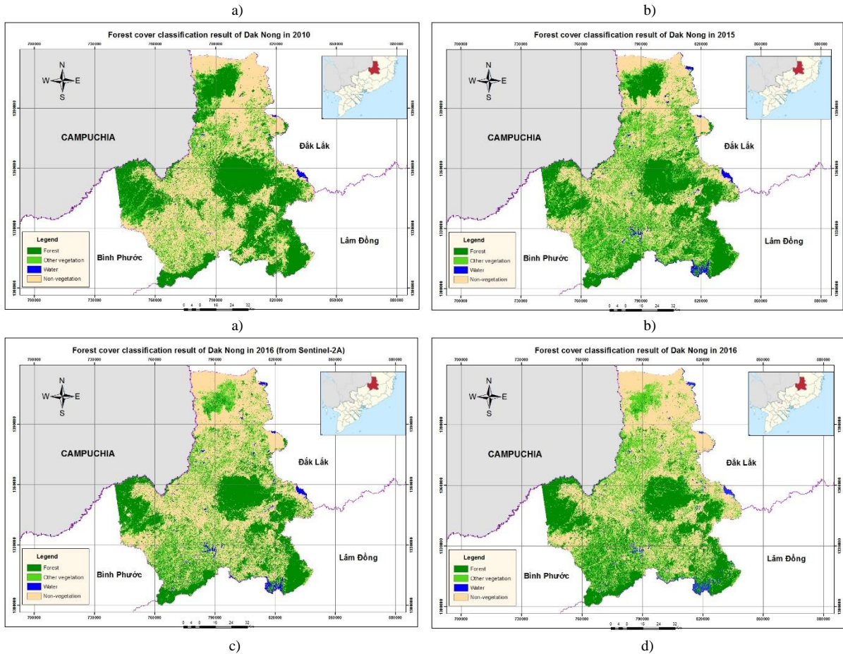
Fig. 3. Forest cover classification results from Landsat-7 2010 (a); Landsat-8 2015 (b); Sentinel-2A 2016 (c); and Landsat-8 2016 (d) images
